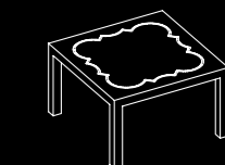
MESA CENTRO CAROLA Medida: 120 x 70 x 35 cm Ref. CAR0901 Medida: 70 x 70 x 42 cm Ref. CAR1001
